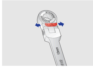
Ratchet: works both ways, turning direction can be changed with button.
